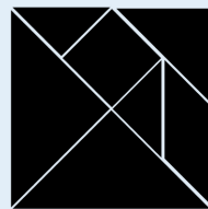
Convex Polygon 1
