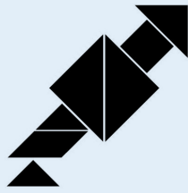
Observatory Telescope
